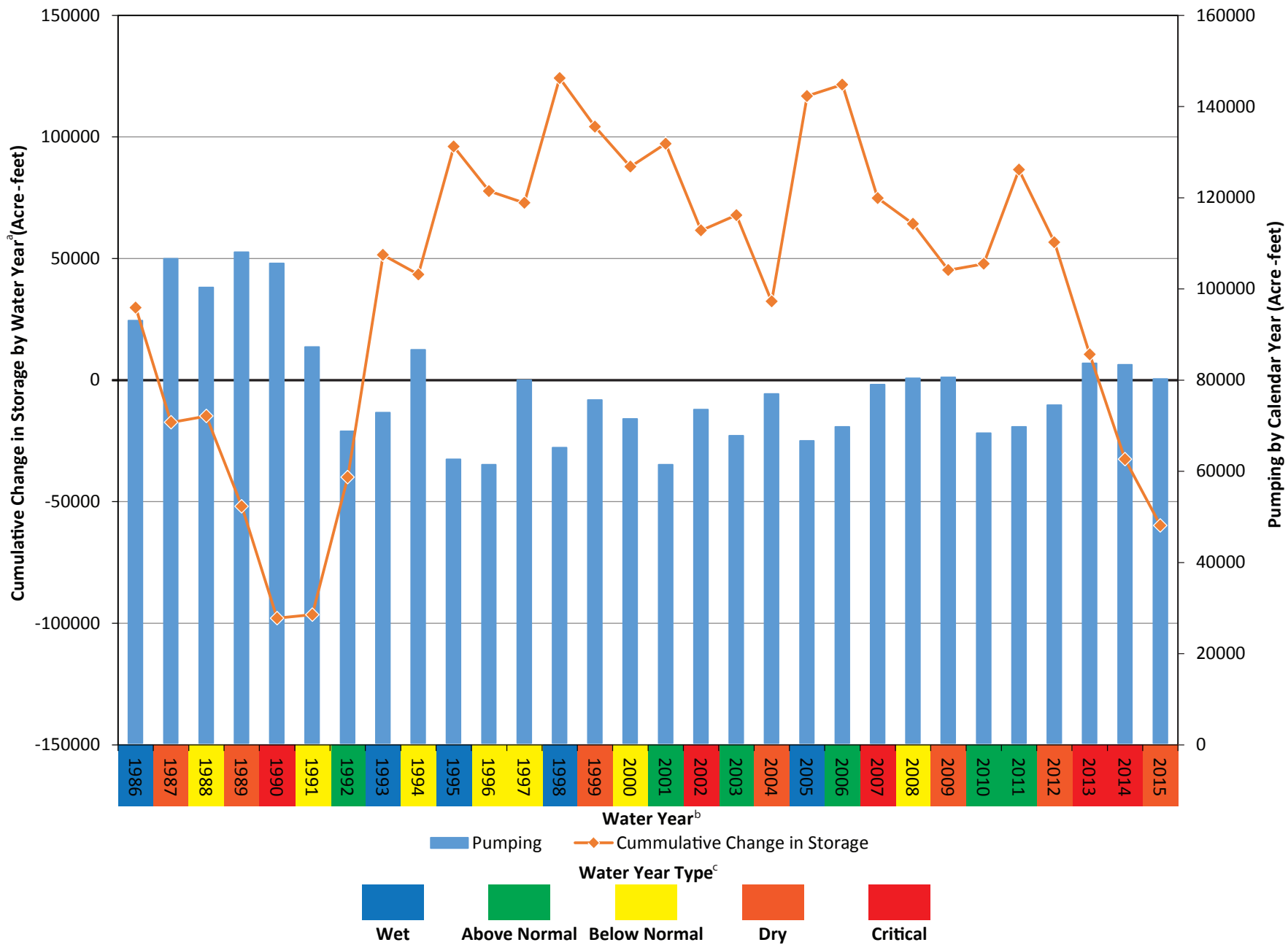
Figure 2-XX Oxnard Subbasin Cumulative Change in Storage
